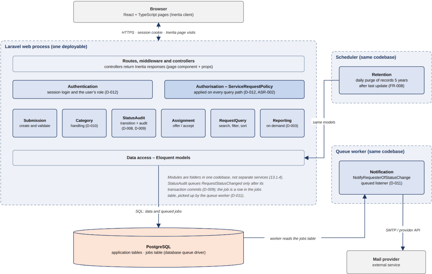
Figure 13.1: CivicConnect logical architecture
